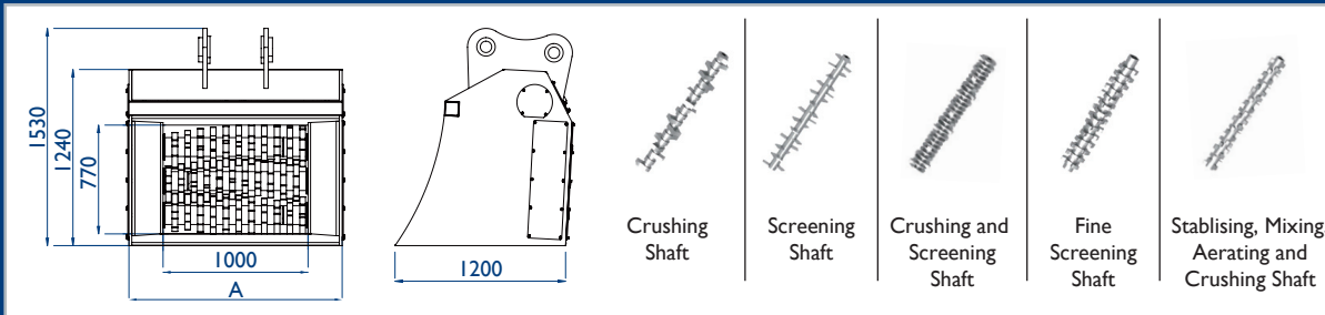
Screening Bucket Attachment Specifications
